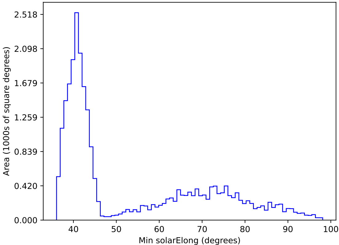
too_ignore_10_4v3.4_10yrs All sky i band: Min solarElong
