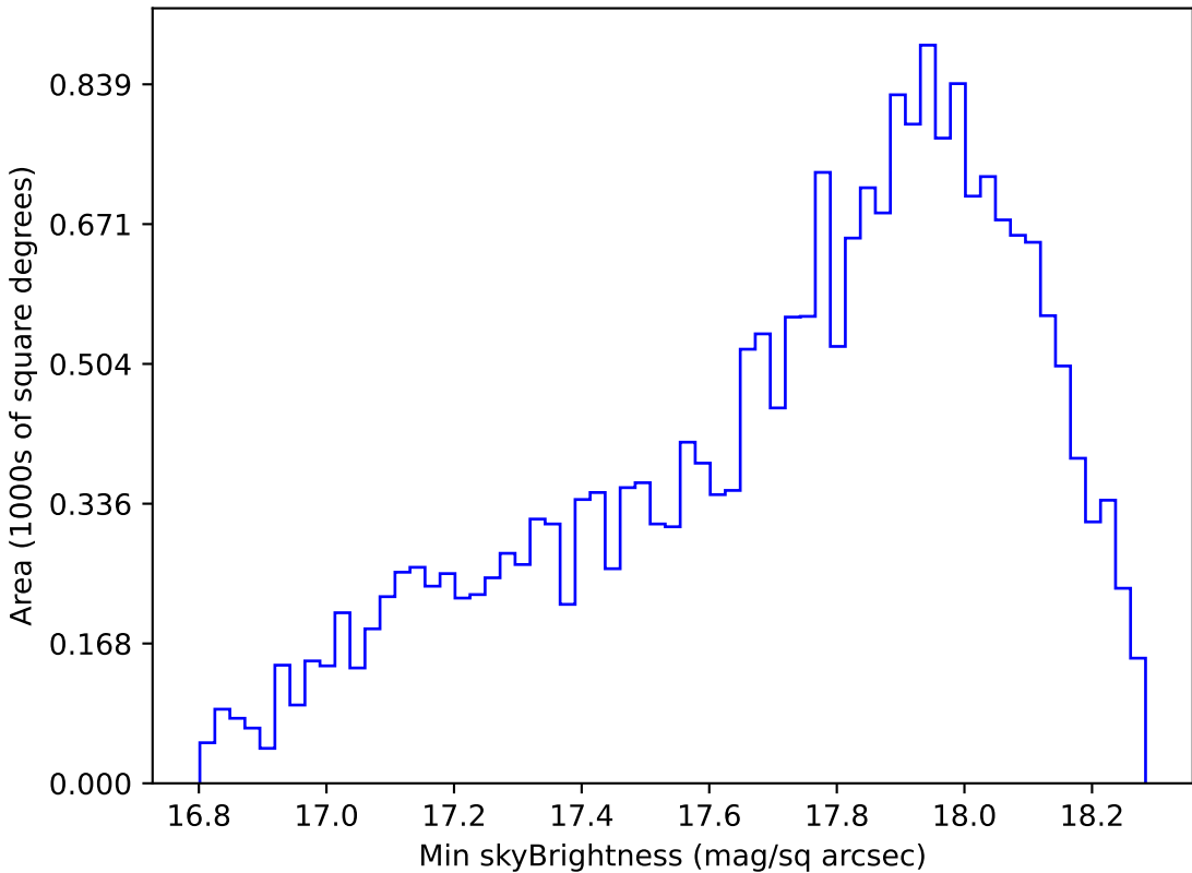
too_ignore_10_4v3.4_10yrs Yr 1 y band: Min skyBrightness
