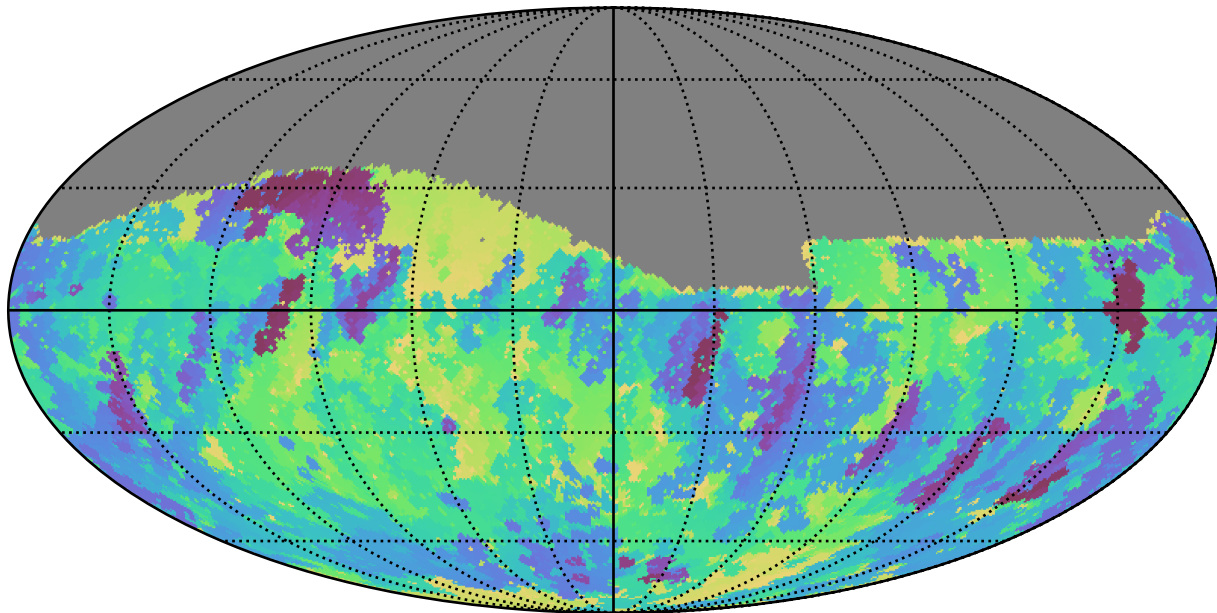
too_ignore_10_4v3.4_10yrs Yr 1 r band: Min skyBrightness
