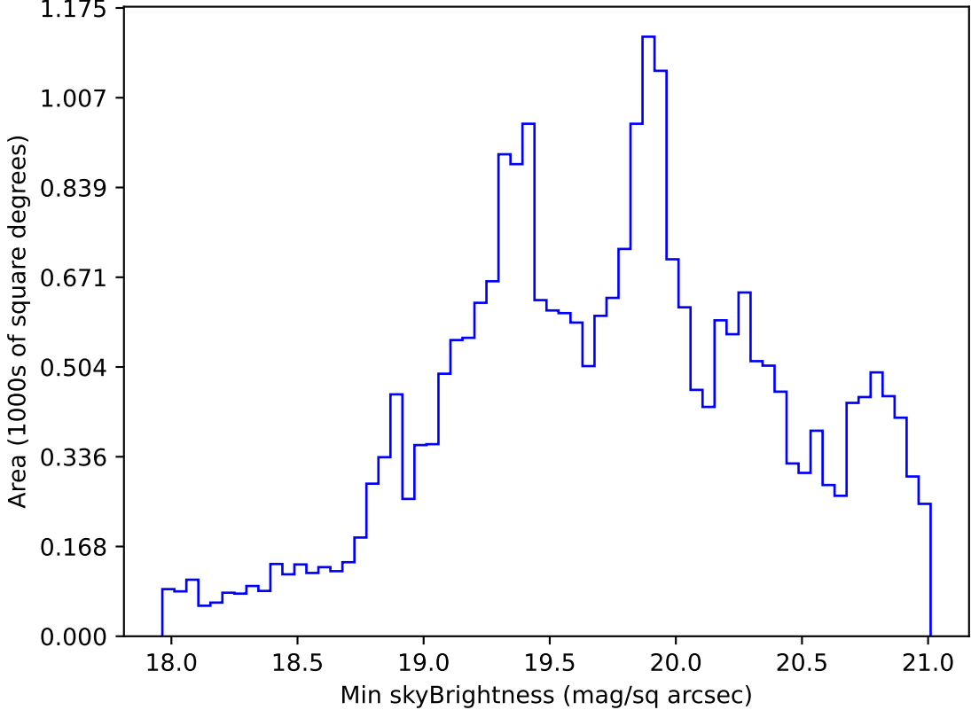
too_ignore_10_4v3.4_10yrs Yr 1 r band: Min skyBrightness
