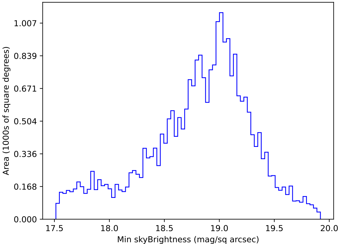
too_ignore_10_4v3.4_10yrs Yr 1 i band: Min skyBrightness
