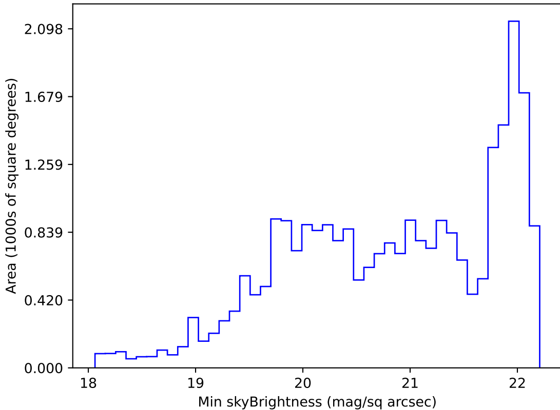
too_ignore_10_4v3.4_10yrs Yr 1 g band: Min skyBrightness
