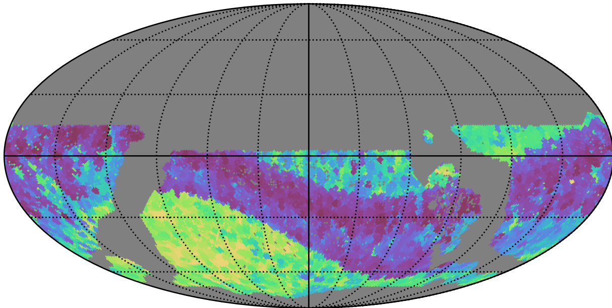
too_ignore_10_4v3.4_10yrs WFD z band: Min skyBrightness
