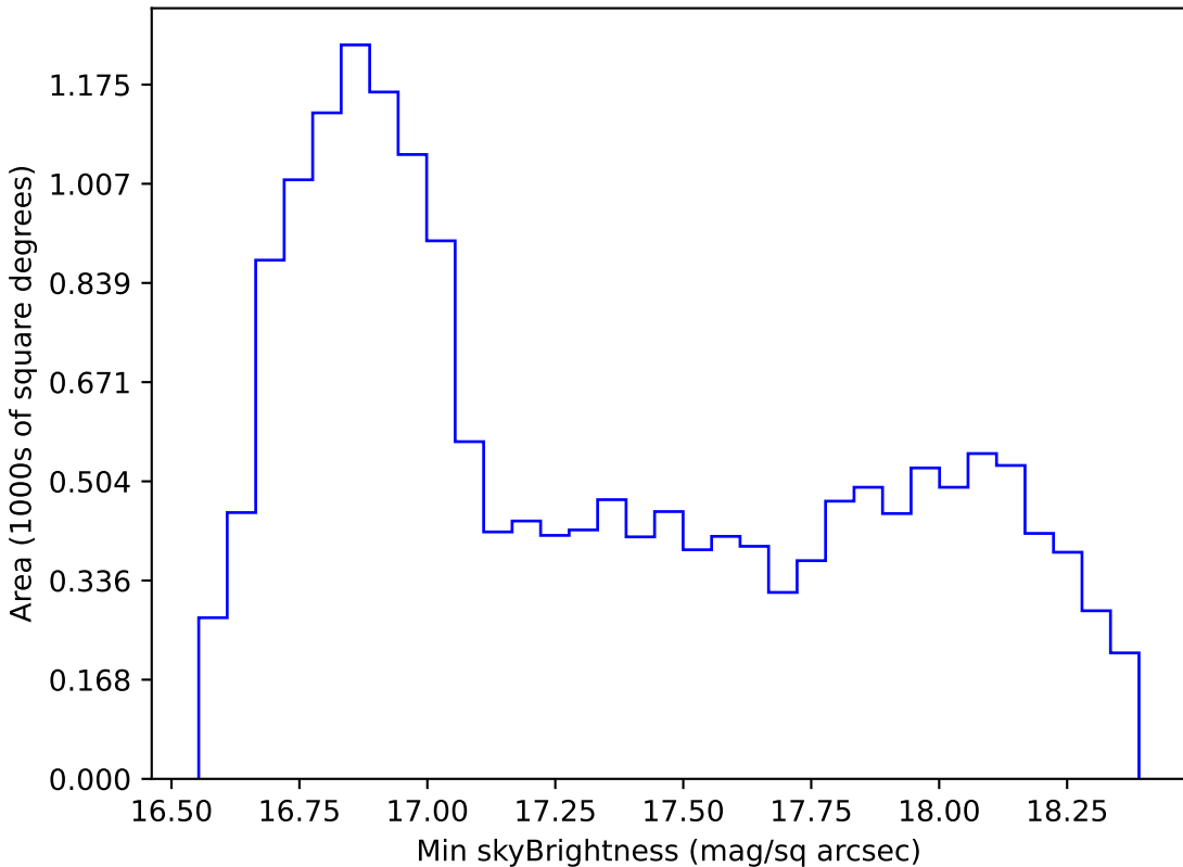
too_ignore_10_4v3.4_10yrs WFD z band: Min skyBrightness
