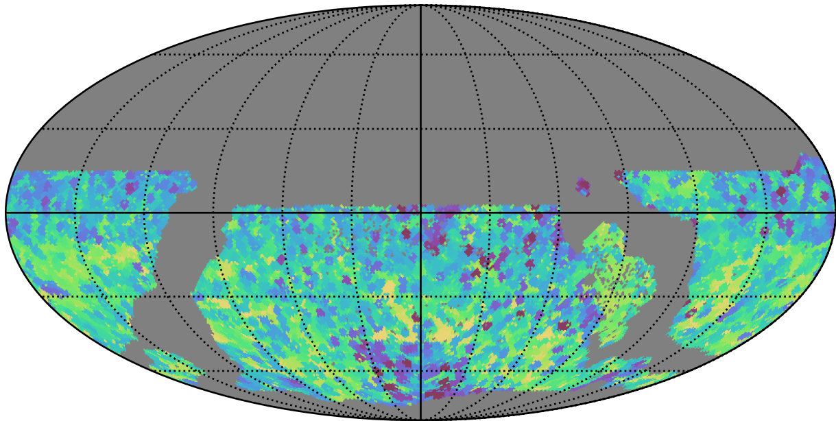
too_ignore_10_4v3.4_10yrs WFD y band: Min skyBrightness
