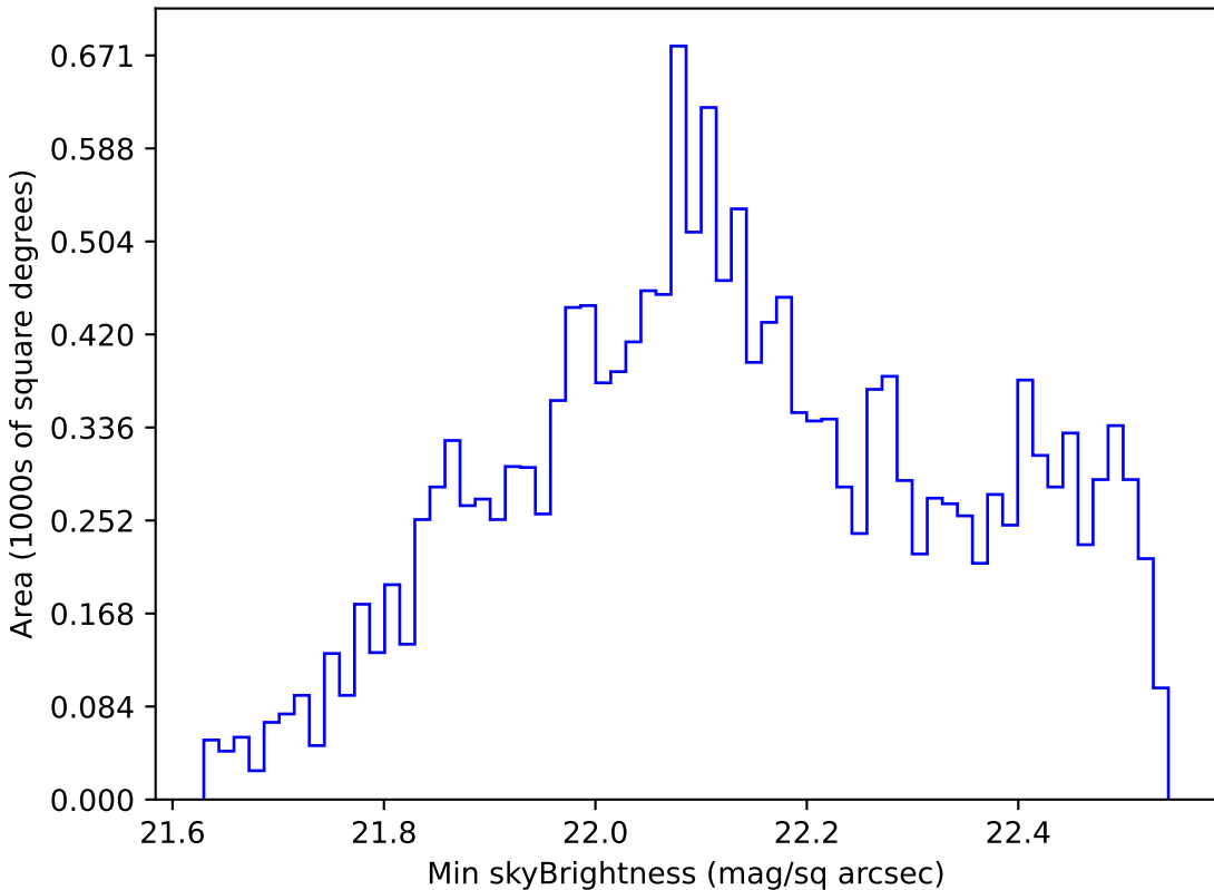
too_ignore_10_4v3.4_10yrs WFD u band: Min skyBrightness
