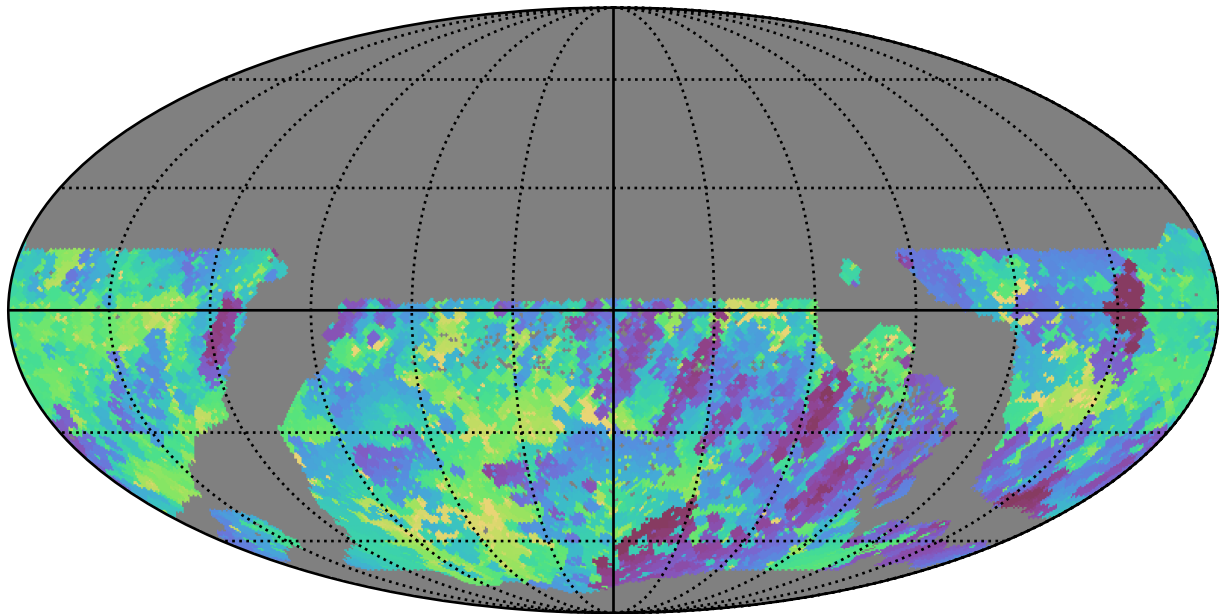
too_ignore_10_4v3.4_10yrs WFD r band: Min skyBrightness
