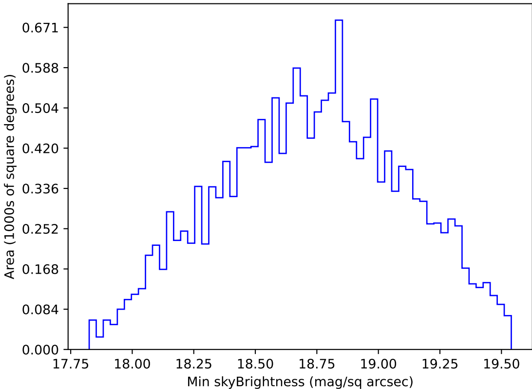
too_ignore_10_4v3.4_10yrs WFD r band: Min skyBrightness
