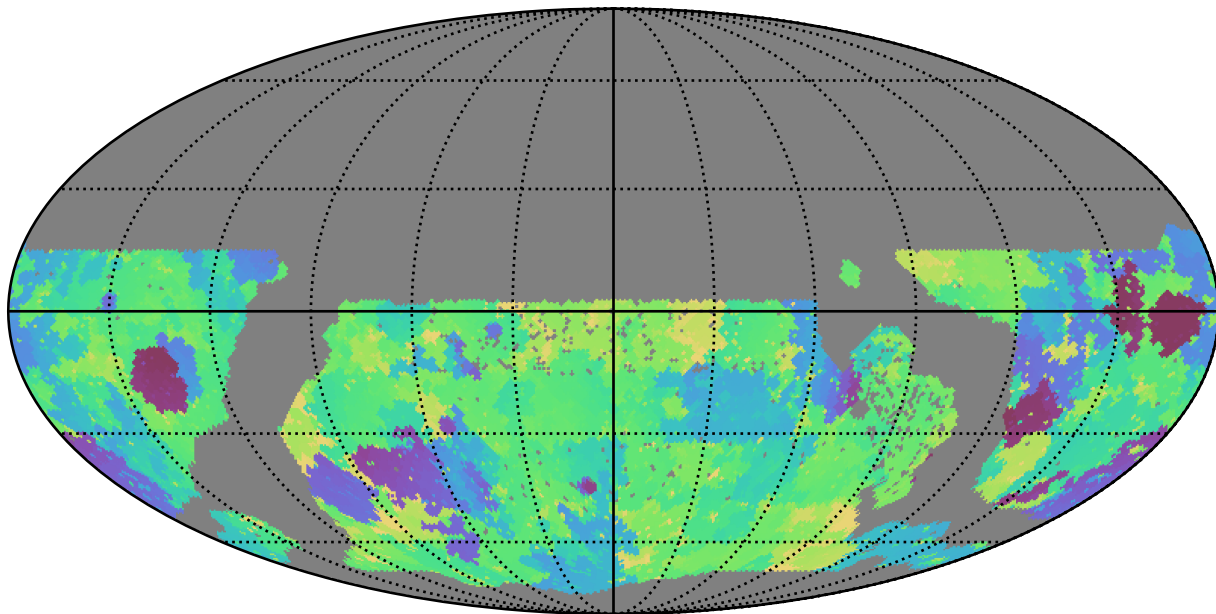
too_ignore_10_4v3.4_10yrs WFD g band: Min skyBrightness
