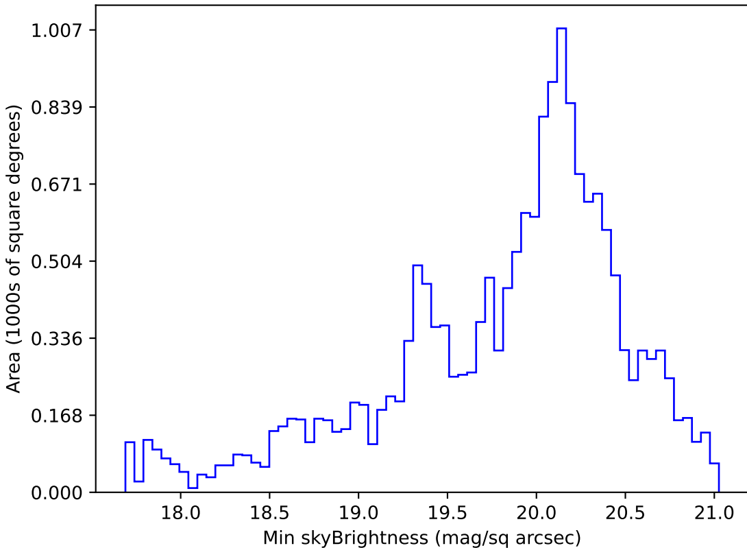
too_ignore_10_4v3.4_10yrs WFD g band: Min skyBrightness
