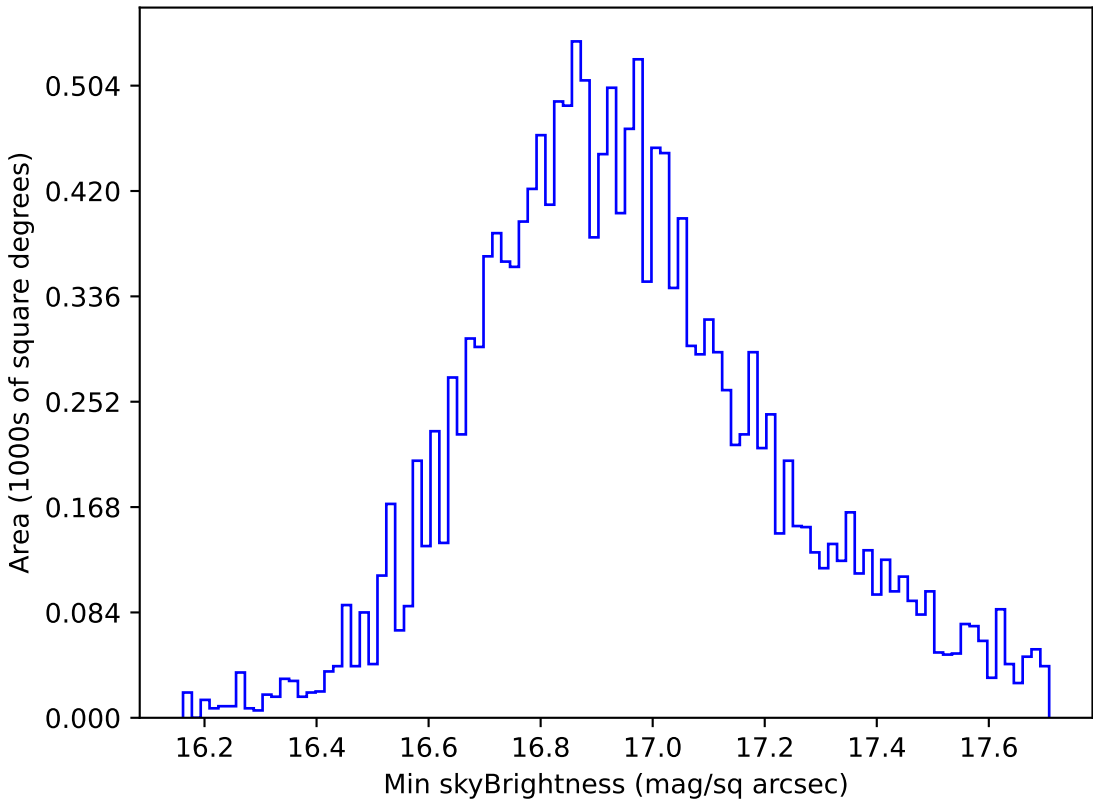
too_ignore_10_4v3.4_10yrs WFD all bands: Min skyBrightness
