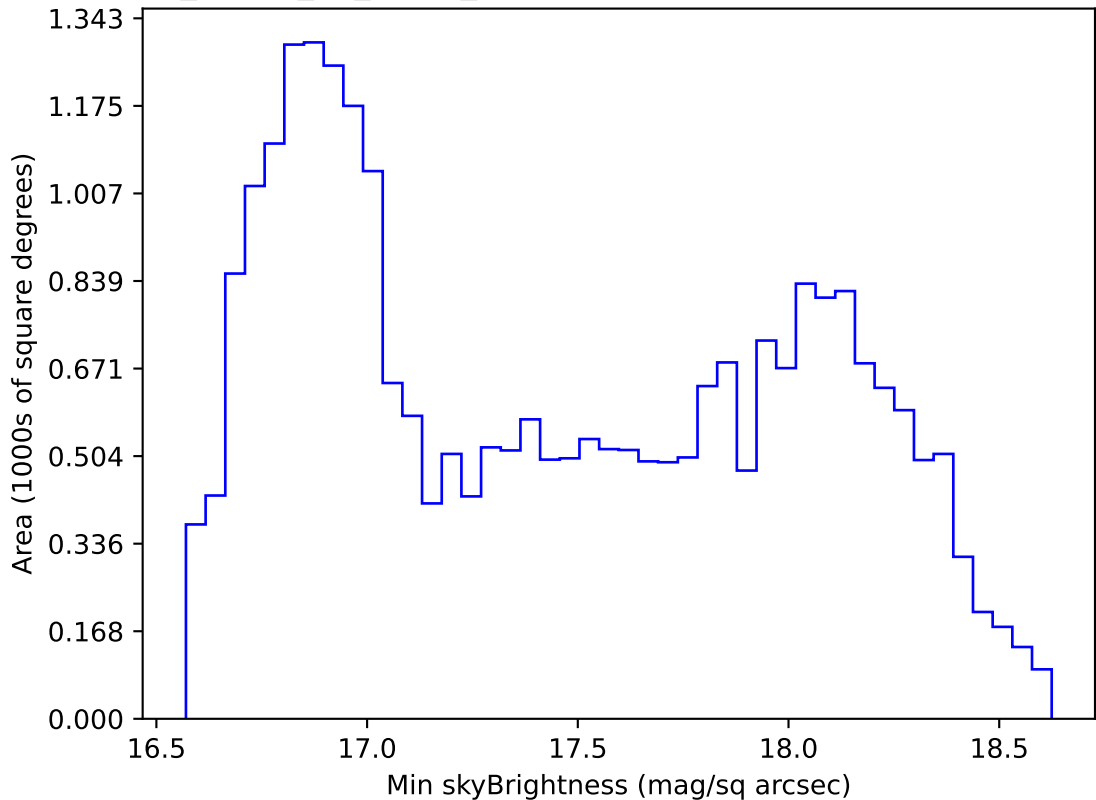
too_ignore_10_4v3.4_10yrs All sky z band: Min skyBrightness
