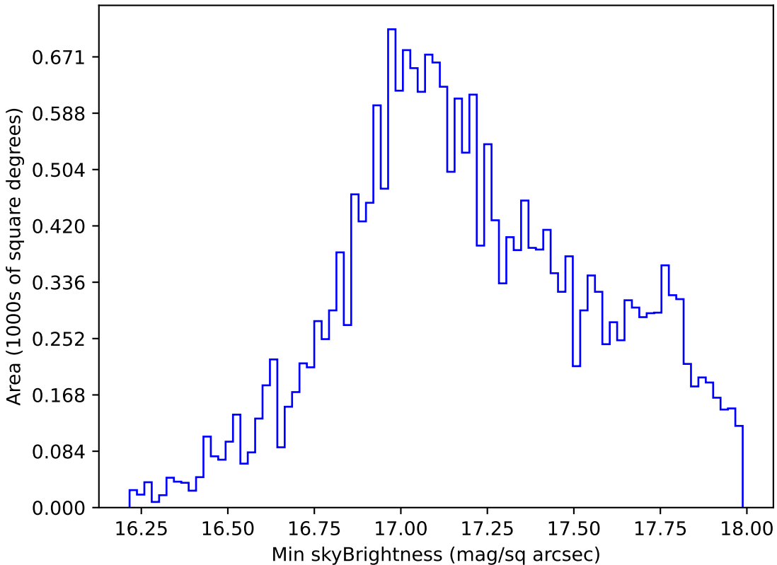
too_ignore_10_4v3.4_10yrs All sky y band: Min skyBrightness
