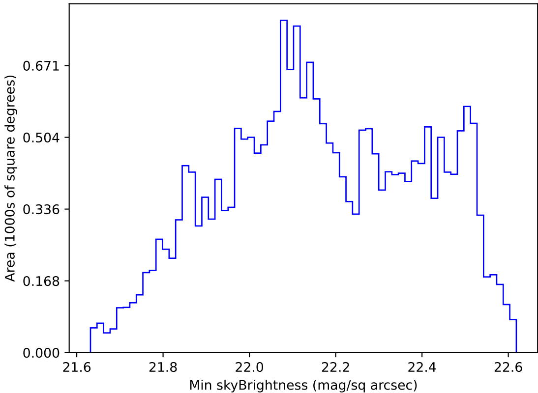
too_ignore_10_4v3.4_10yrs All sky u band: Min skyBrightness
