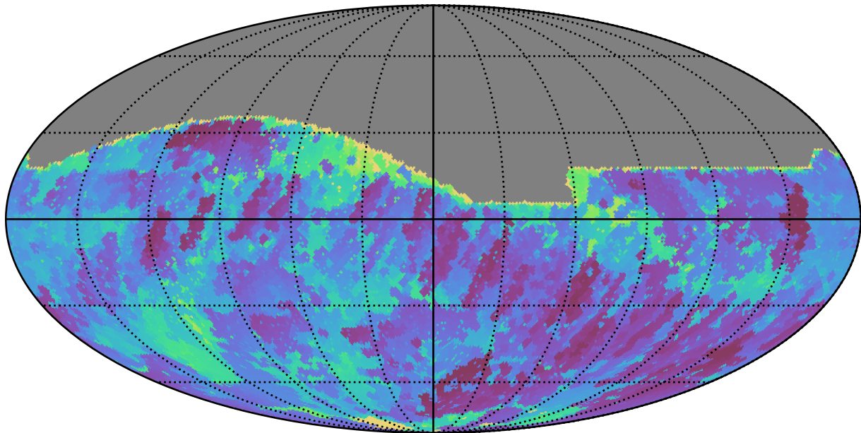
too_ignore_10_4v3.4_10yrs All sky r band: Min skyBrightness
