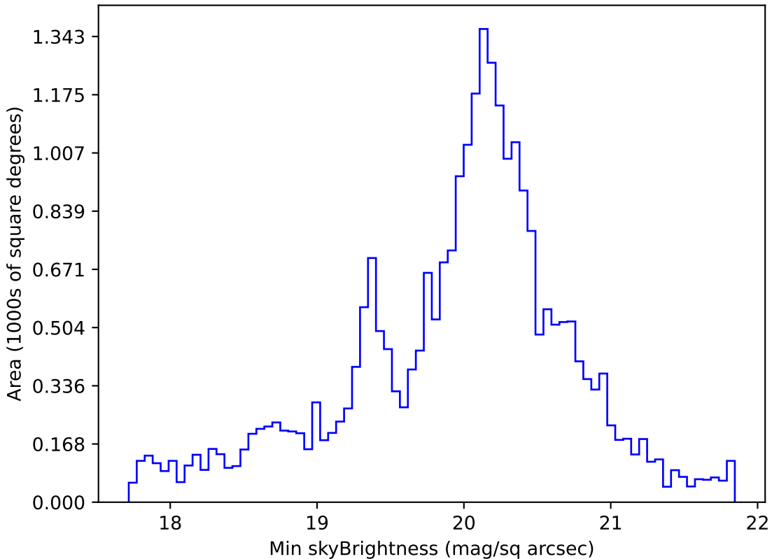
too_ignore_10_4v3.4_10yrs All sky g band: Min skyBrightness
