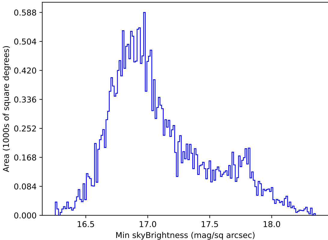
too_ignore_10_4v3.4_10yrs All sky all bands: Min skyBrightness
