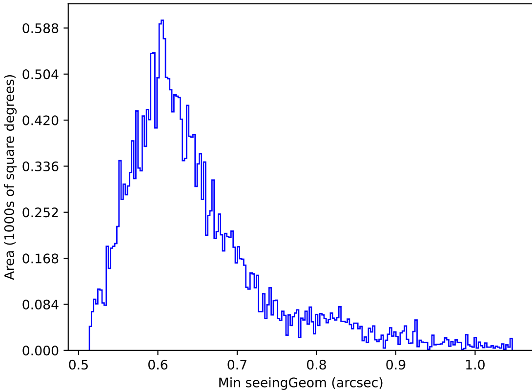
too_ignore_10_4v3.4_10yrs Yr 1 z band: Min seeingGeom
