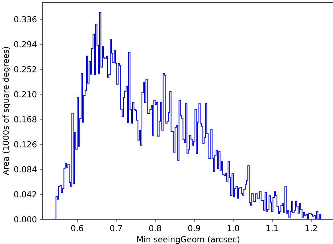
too_ignore_10_4v3.4_10yrs Yr 1 u band: Min seeingGeom
