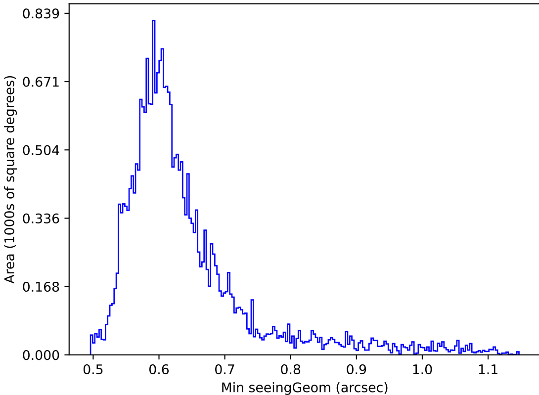
too_ignore_10_4v3.4_10yrs Yr 1 i band: Min seeingGeom
