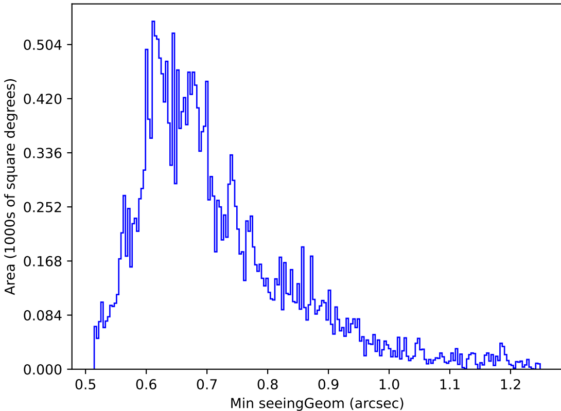
too_ignore_10_4v3.4_10yrs Yr 1 g band: Min seeingGeom
