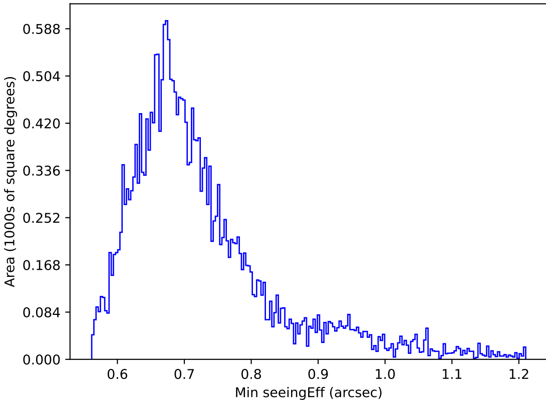
too_ignore_10_4v3.4_10yrs Yr 1 z band: Min seeingEff
