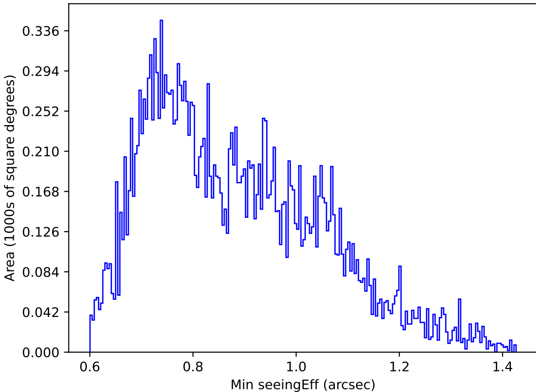
too_ignore_10_4v3.4_10yrs Yr 1 u band: Min seeingEff
