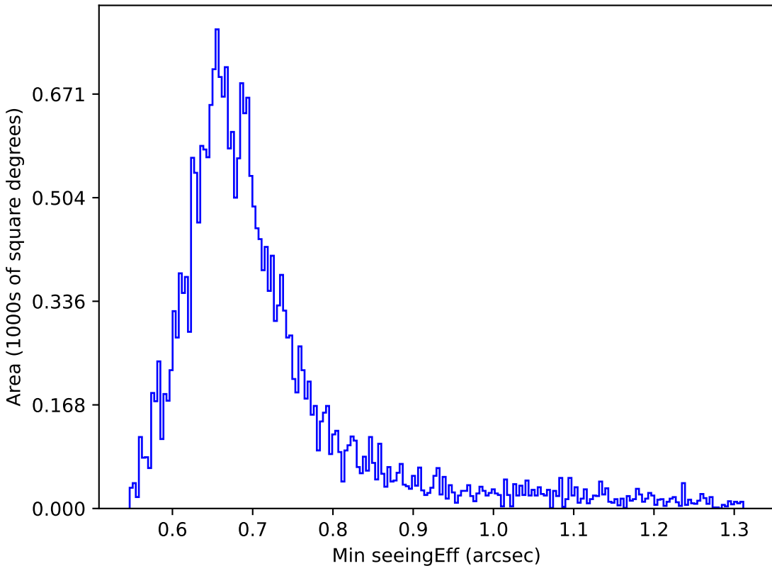
too_ignore_10_4v3.4_10yrs Yr 1 r band: Min seeingEff
