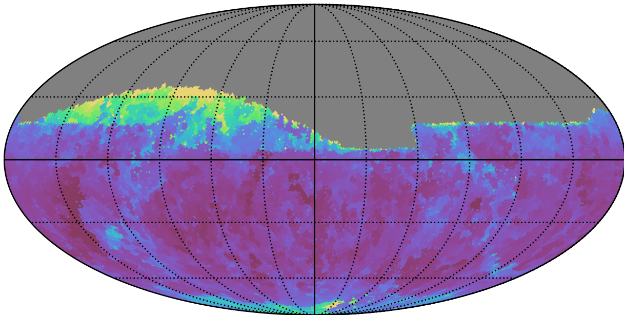
too_ignore_10_4v3.4_10yrs Yr 1 i band: Min seeingEff
