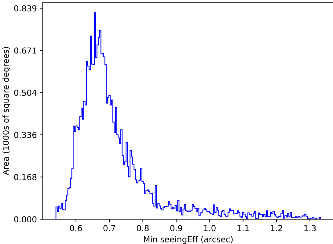
too_ignore_10_4v3.4_10yrs Yr 1 i band: Min seeingEff
