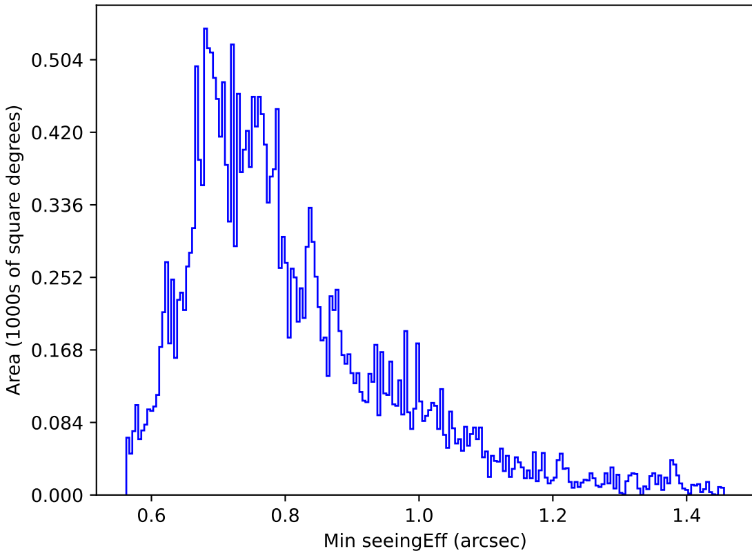
too_ignore_10_4v3.4_10yrs Yr 1 g band: Min seeingEff
