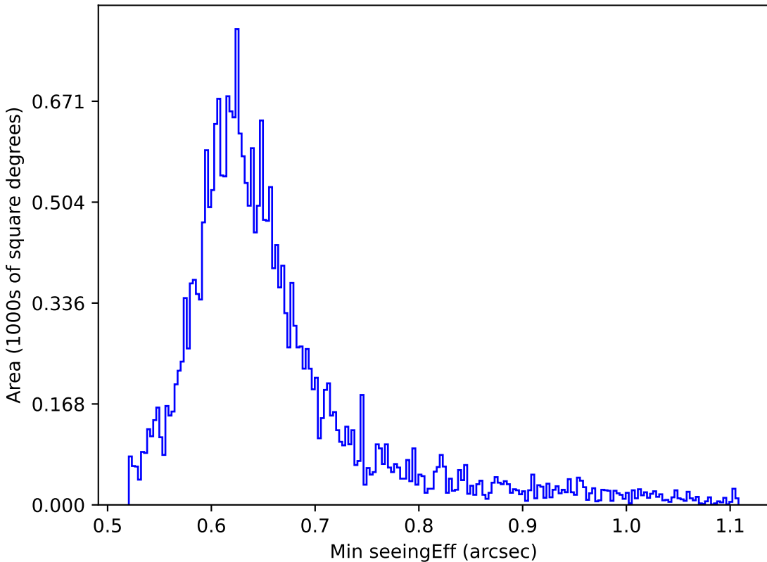
too_ignore_10_4v3.4_10yrs Yr 1 all bands: Min seeingEff
