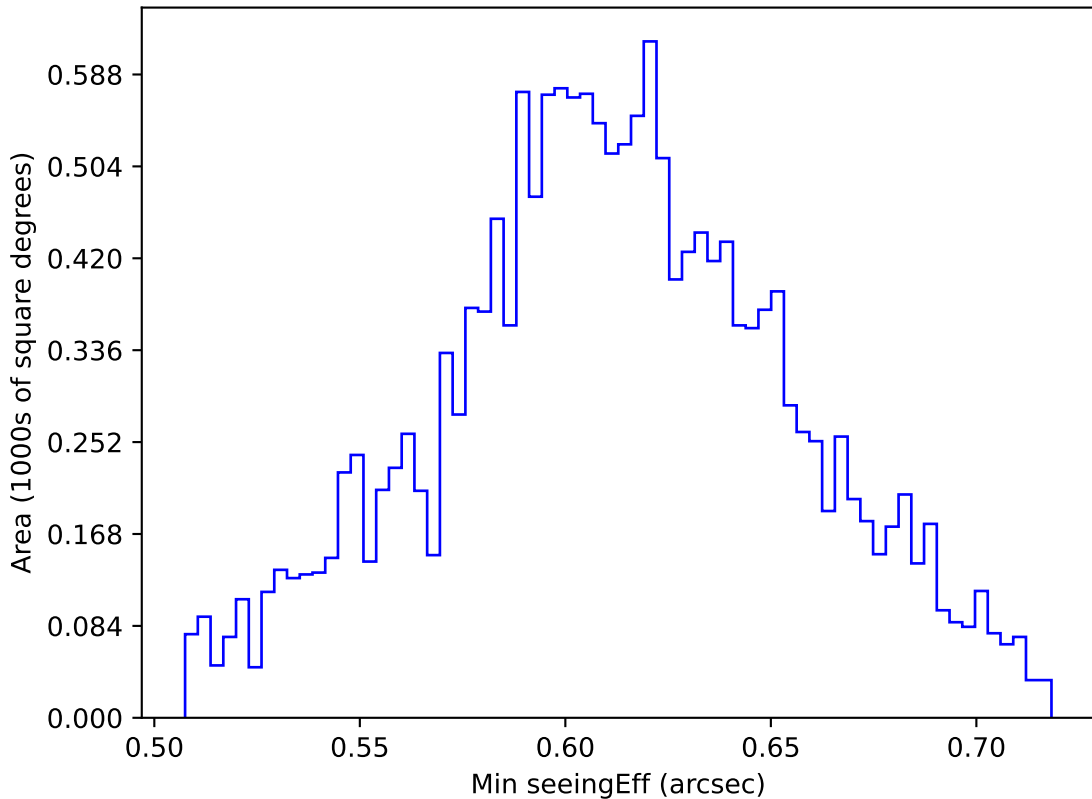
too_ignore_10_4v3.4_10yrs WFD z band: Min seeingEff
