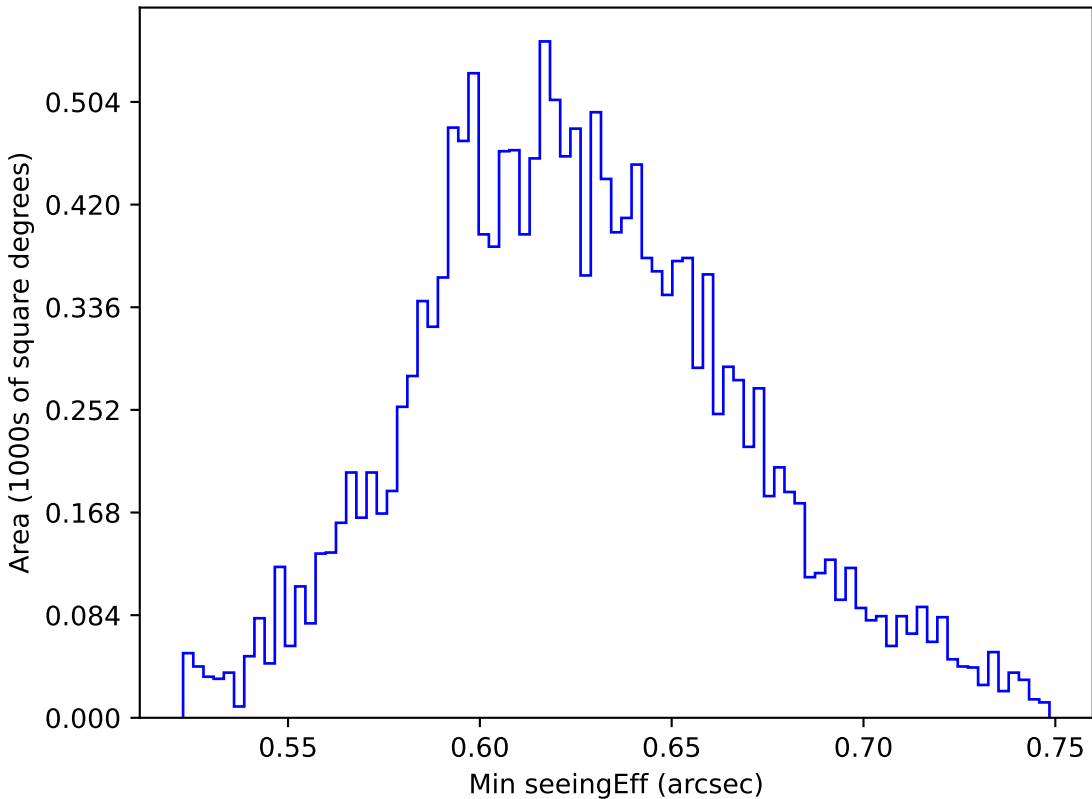
too_ignore_10_4v3.4_10yrs WFD y band: Min seeingEff
