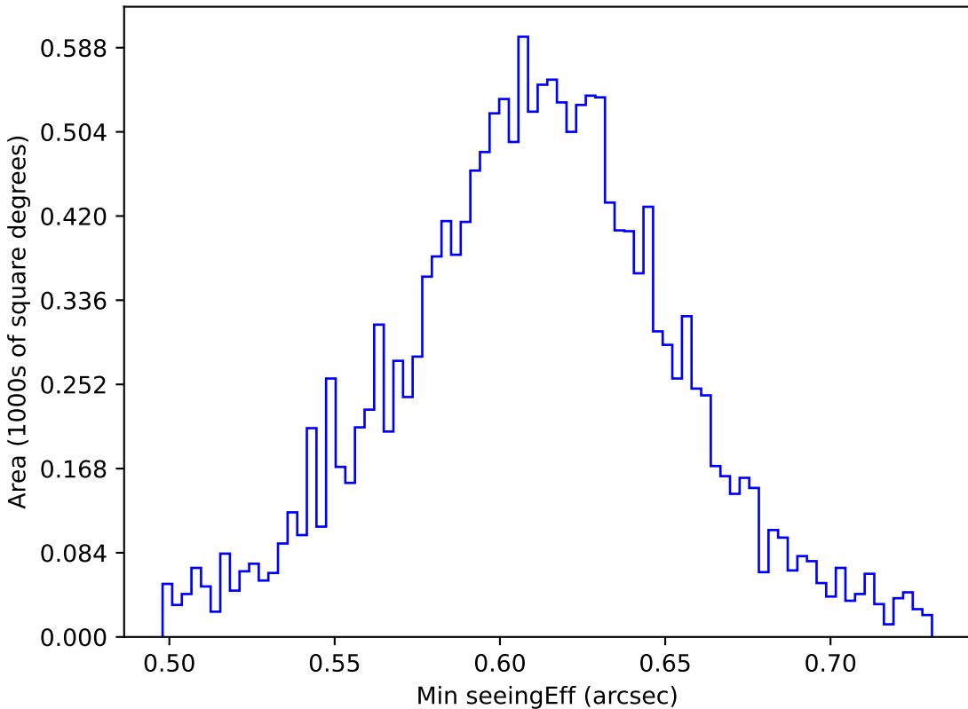
too_ignore_10_4v3.4_10yrs WFD r band: Min seeingEff
