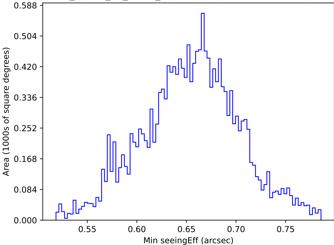
too_ignore_10_4v3.4_10yrs WFD g band: Min seeingEff
