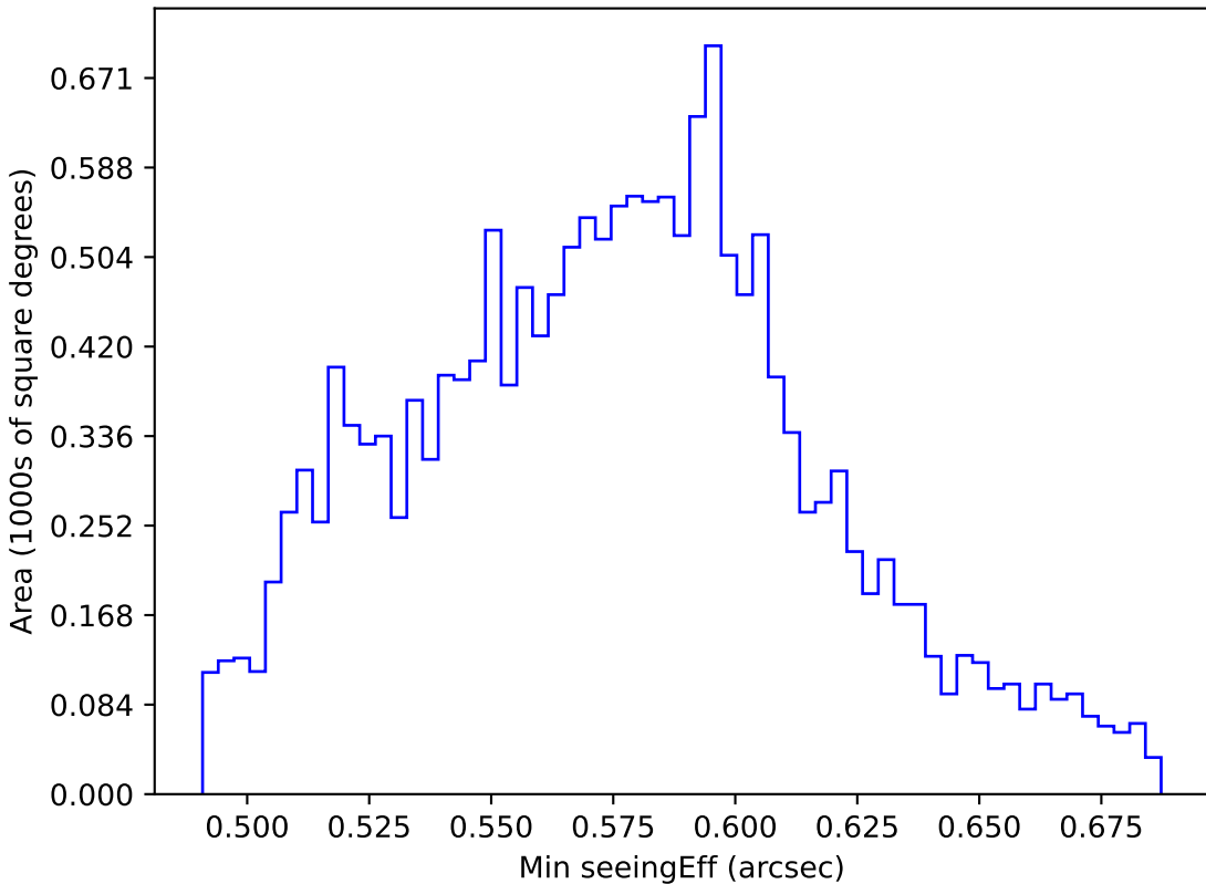
too_ignore_10_4v3.4_10yrs WFD all bands: Min seeingEff
