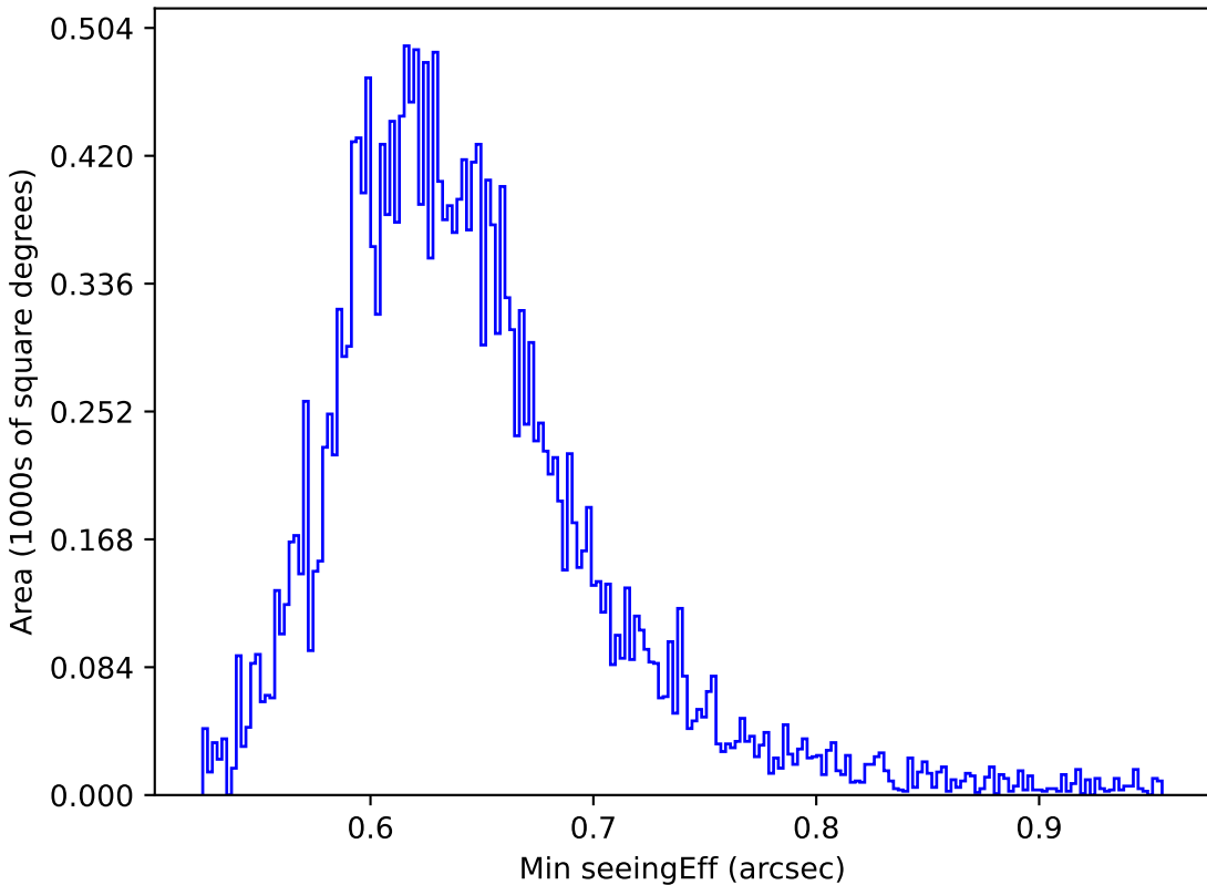
too_ignore_10_4v3.4_10yrs All sky y band: Min seeingEff
