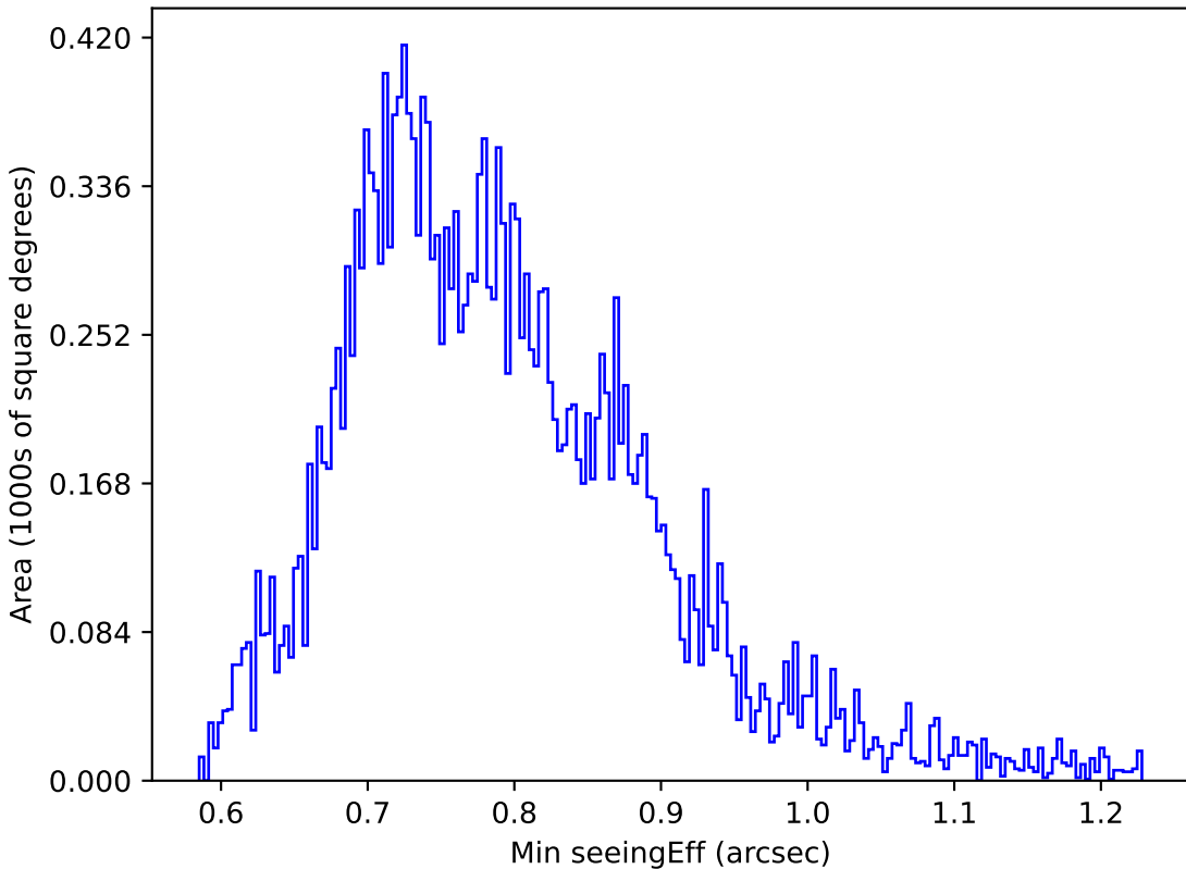
too_ignore_10_4v3.4_10yrs All sky u band: Min seeingEff
