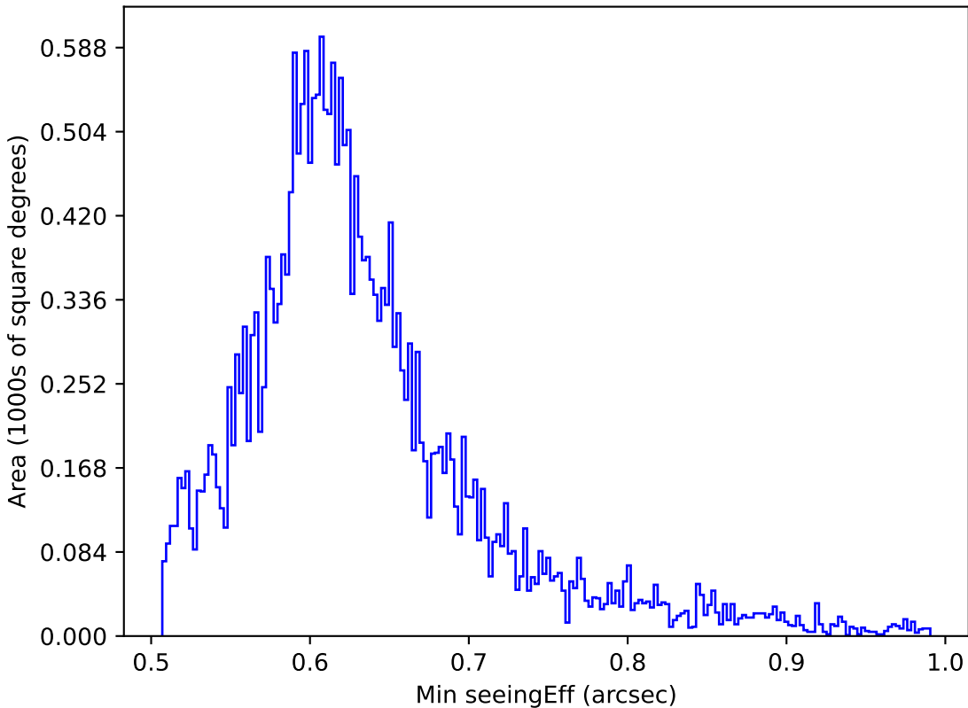
too_ignore_10_4v3.4_10yrs All sky i band: Min seeingEff
