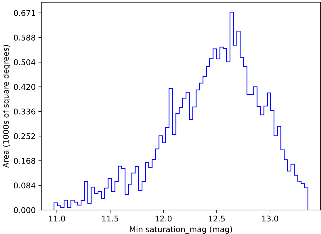
too_ignore_10_4v3.4_10yrs WFD r band: Min saturation_mag
