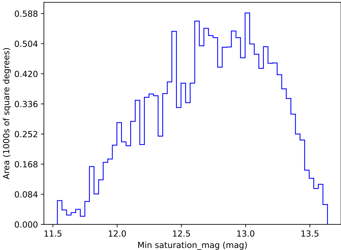
too_ignore_10_4v3.4_10yrs WFD g band: Min saturation_mag
