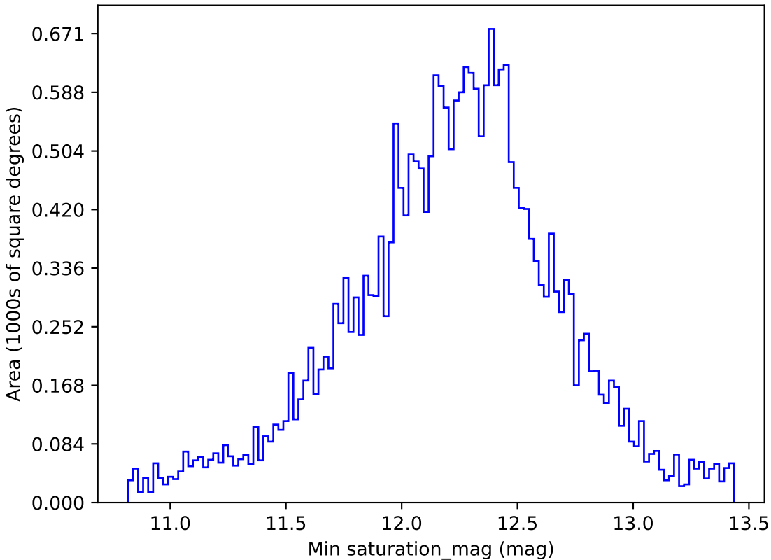
too_ignore_10_4v3.4_10yrs All sky z band: Min saturation_mag
