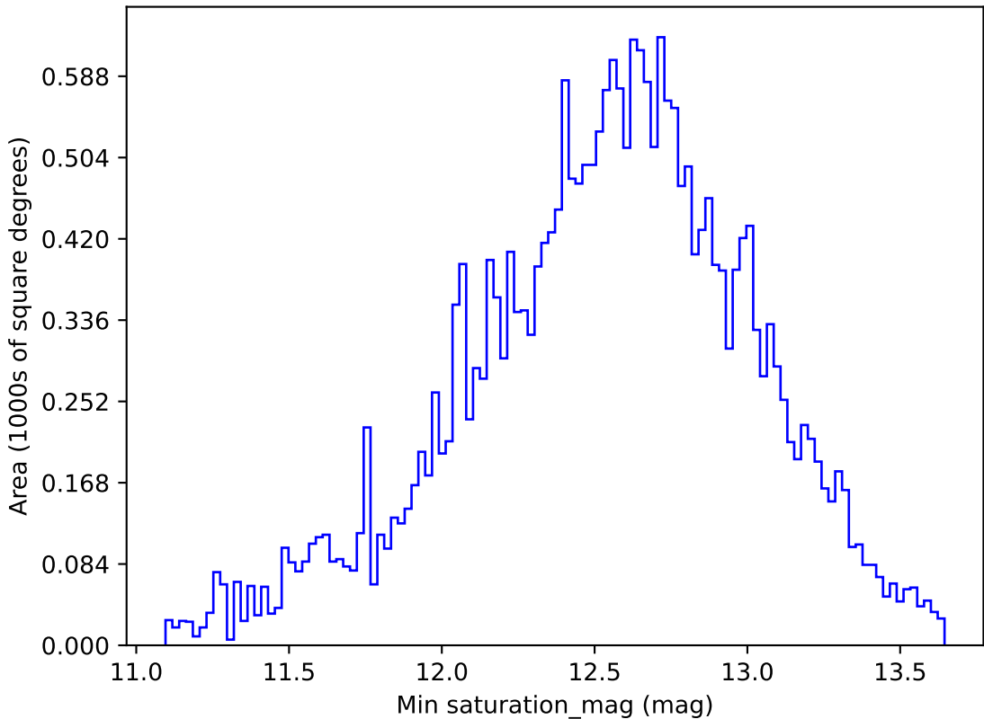
too_ignore_10_4v3.4_10yrs All sky r band: Min saturation_mag
