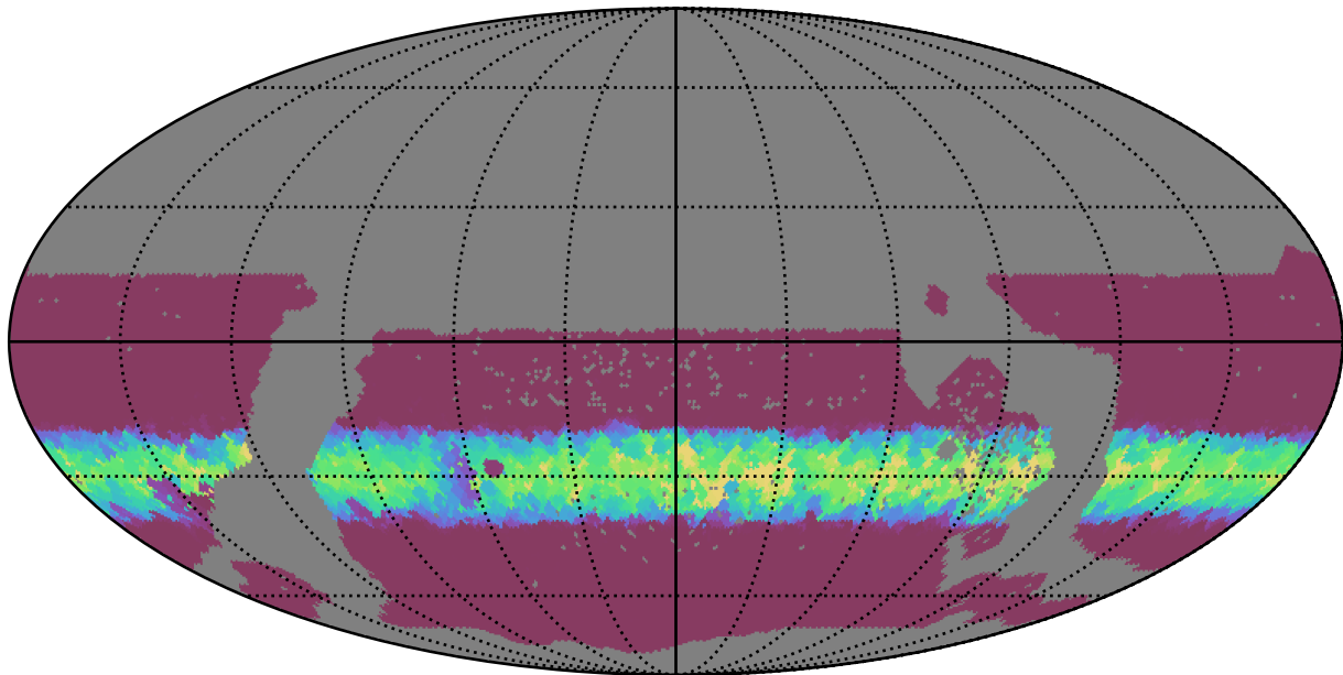
too_ignore_10_4v3.4_10yrs WFD z band: Min normairmass
