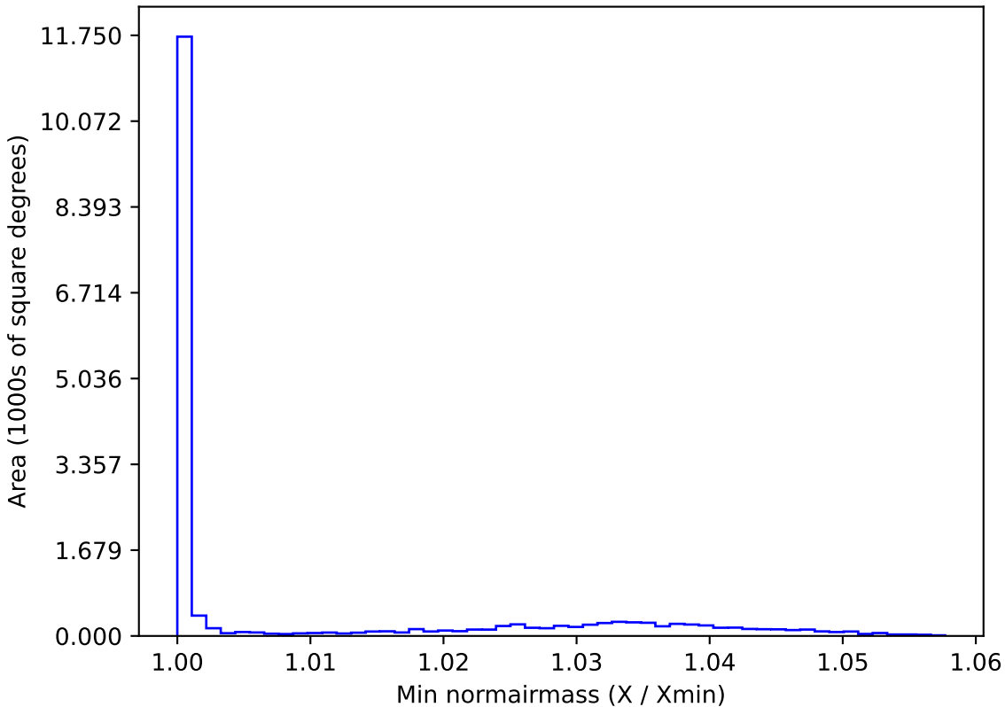
too_ignore_10_4v3.4_10yrs WFD u band: Min normairmass
