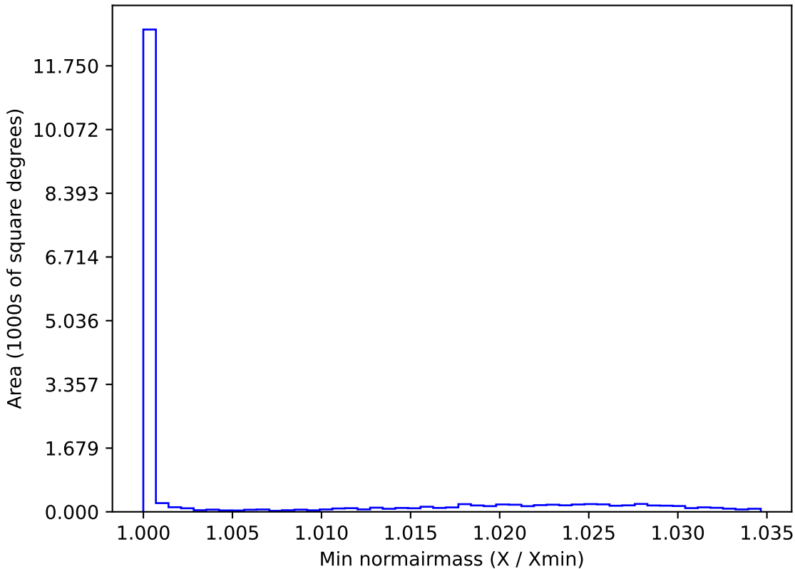
too_ignore_10_4v3.4_10yrs WFD r band: Min normairmass
