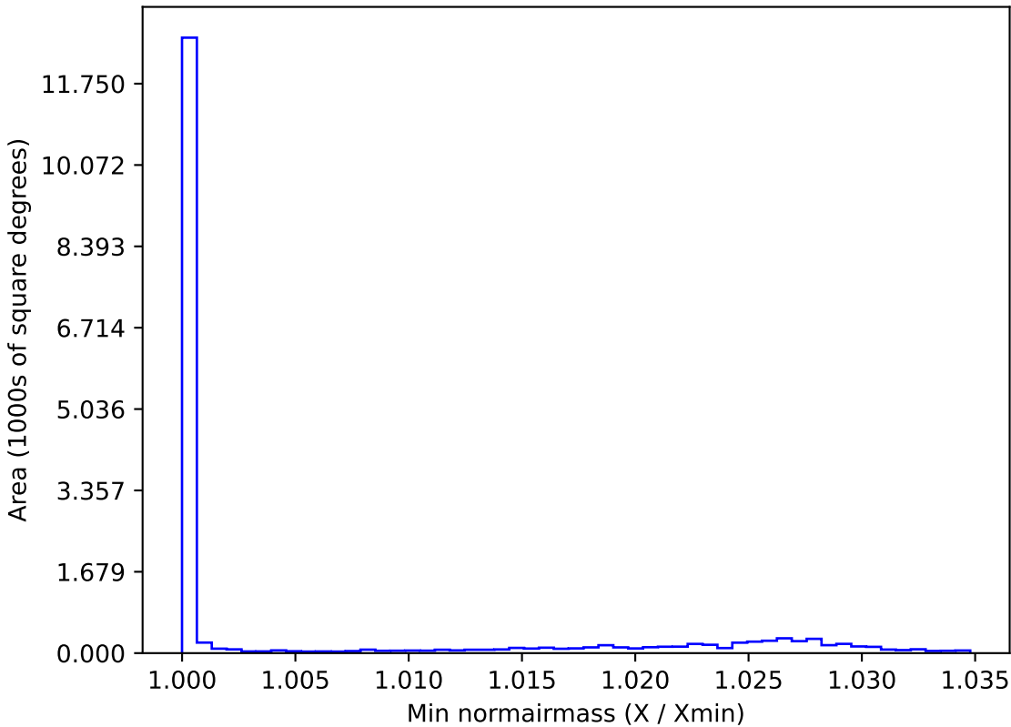
too_ignore_10_4v3.4_10yrs WFD i band: Min normairmass
