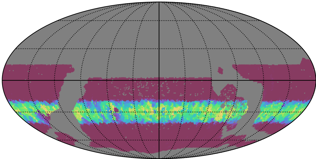
too_ignore_10_4v3.4_10yrs WFD g band: Min normairmass
