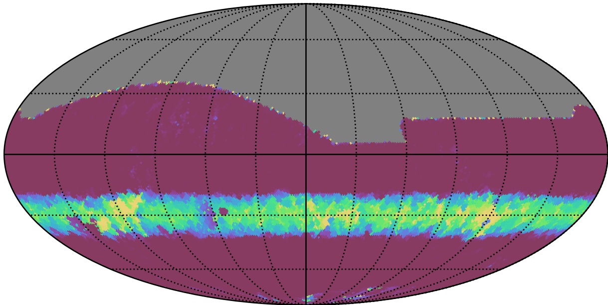
too_ignore_10_4v3.4_10yrs All sky z band: Min normairmass
